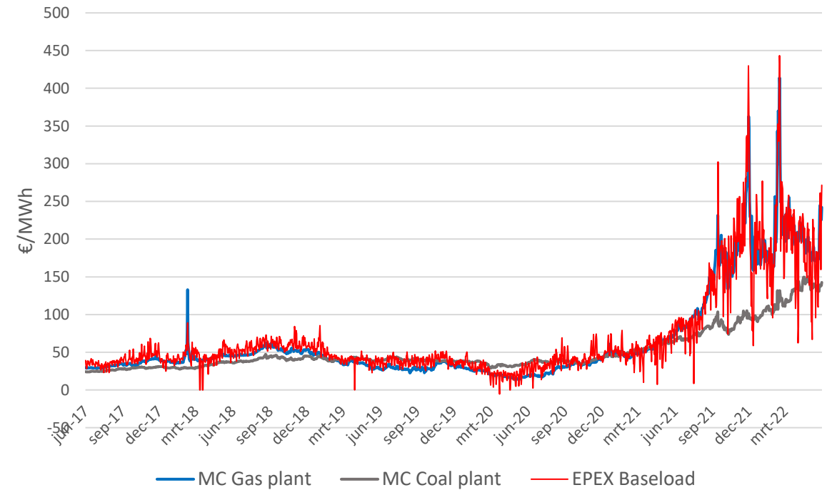
Marginal costs gas & coal plants and average daily EPEX prices
